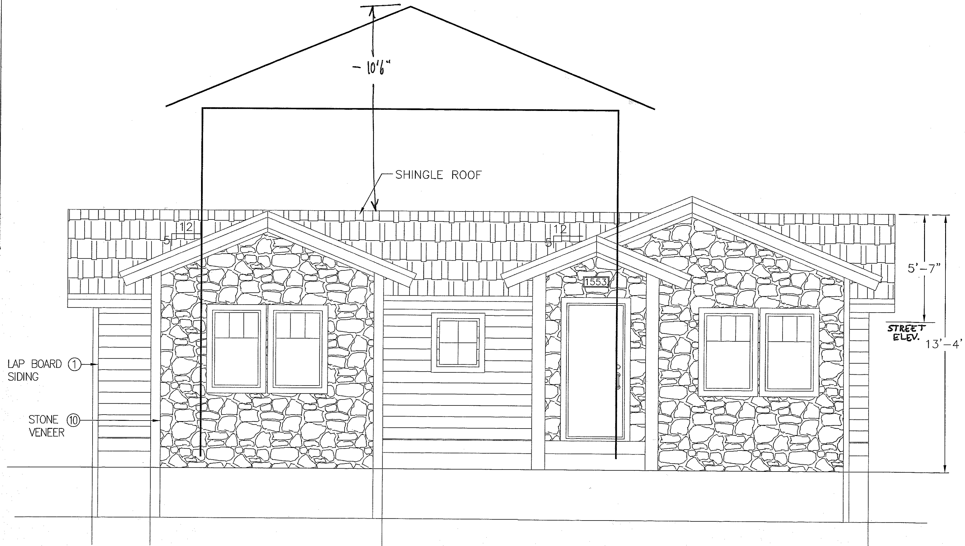
SOUTH ELEVATION
